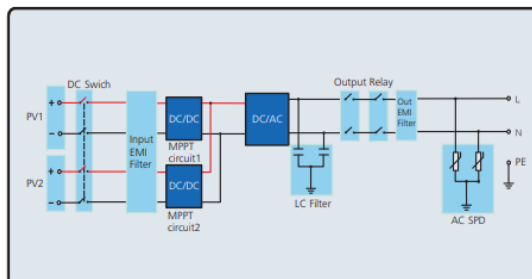
Growatt 3.6-5.5MTL-S topologia
